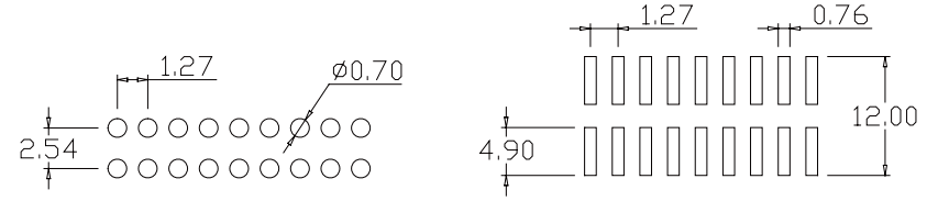
Recommended PCB Layout (PCB TOLERANCE±0.05)
